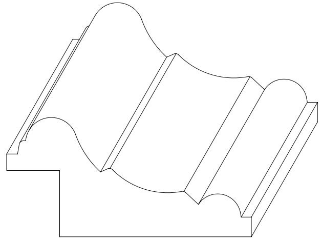
W-1704 1 1/8" x 2 5/16" *1/2" x 5/8" RABBET
