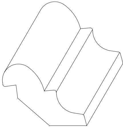
W-937 5/8" x 1 11/16" *1/4" x 3/4" RABBET
