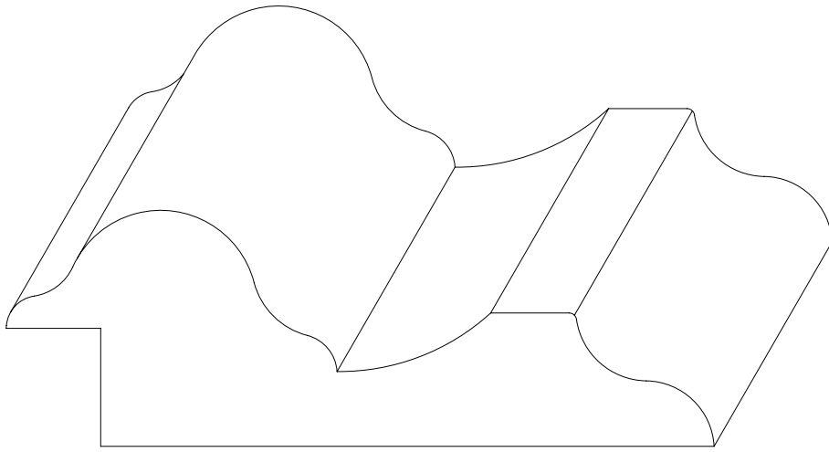
W-1703 1 1/4" x 3 3/4" *1/2" x 5/8" RABBET
