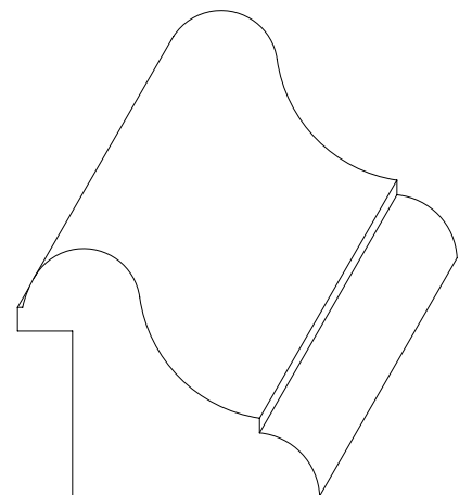
W-1157 1 1/8" x 1 3/8" *1/4" x 3/4" RABBET
