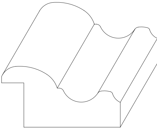
W-953A 1 1/32" x 2" *3/8" x 3/4" RABBET
