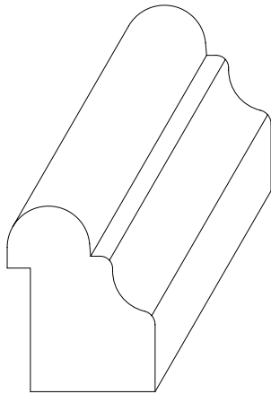
W-1711 1" x 13/16" *1/8" x 5/8" RABBET
