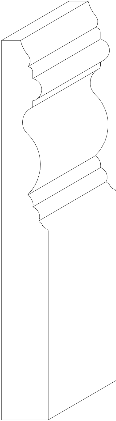
W-249 3/4" x 4 1/4" - 7 1/4"
