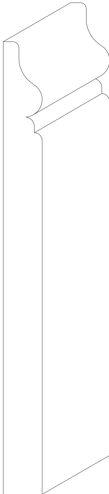
W-112A 5/8" x 7 1/4"
