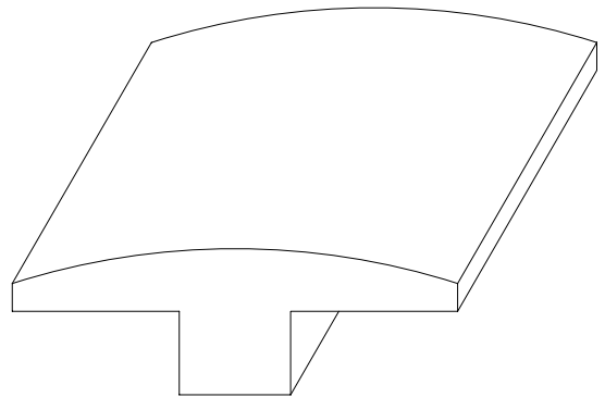
W-1872 21/32" x 2"
