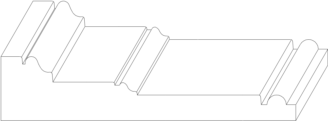
W-1892 1 1/4" x 5 3/4"
