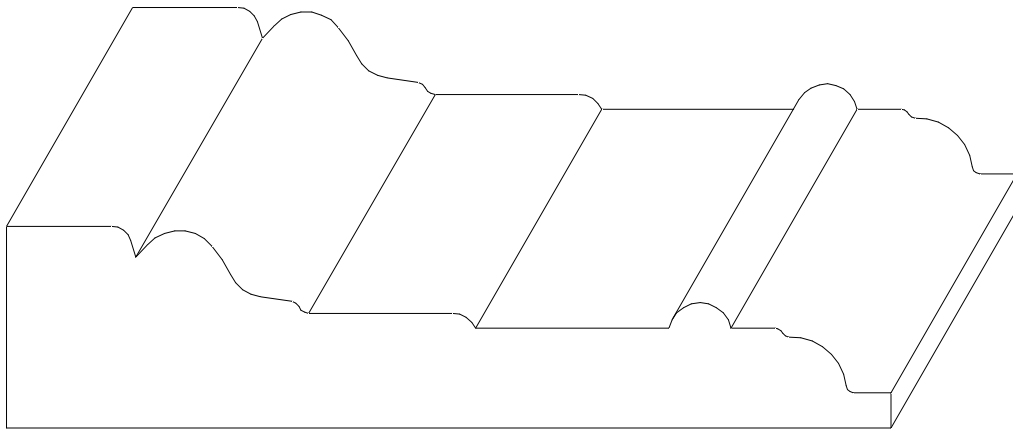
W-1221 1" x 4 3/8"
