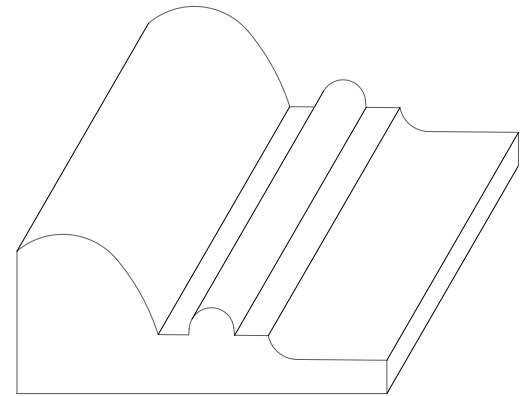
W-2343 13/16" x 1-3/4"
