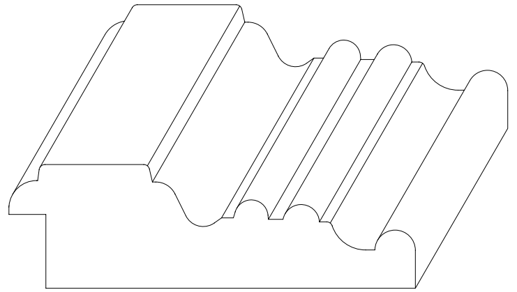
W-2122 13/16" x 2 3/4"
