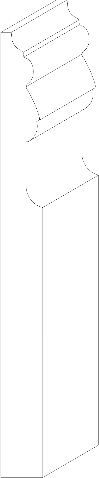
W-2366 13/16" x 8-1/2"
