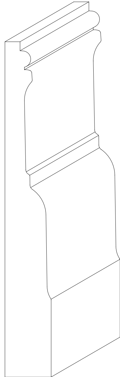
W-2387 3/4" x 5-1/4"
