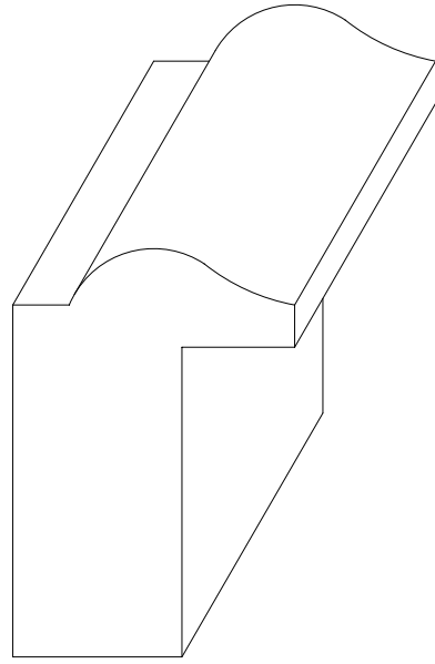
W-1483 1 13/16" x 1 1/4" * 1/2" x 1 3/8" RABBET
