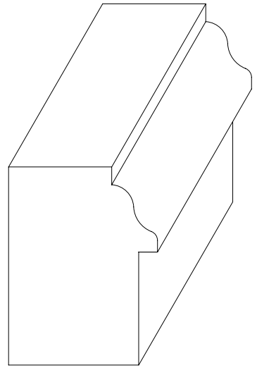
W-2404 1-5/16" x 1" * 1/8" x 3/4" RABBET
