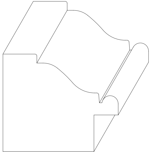
W-793 2" x 2 3/8" * 1/2" x 3/4" RABBET
