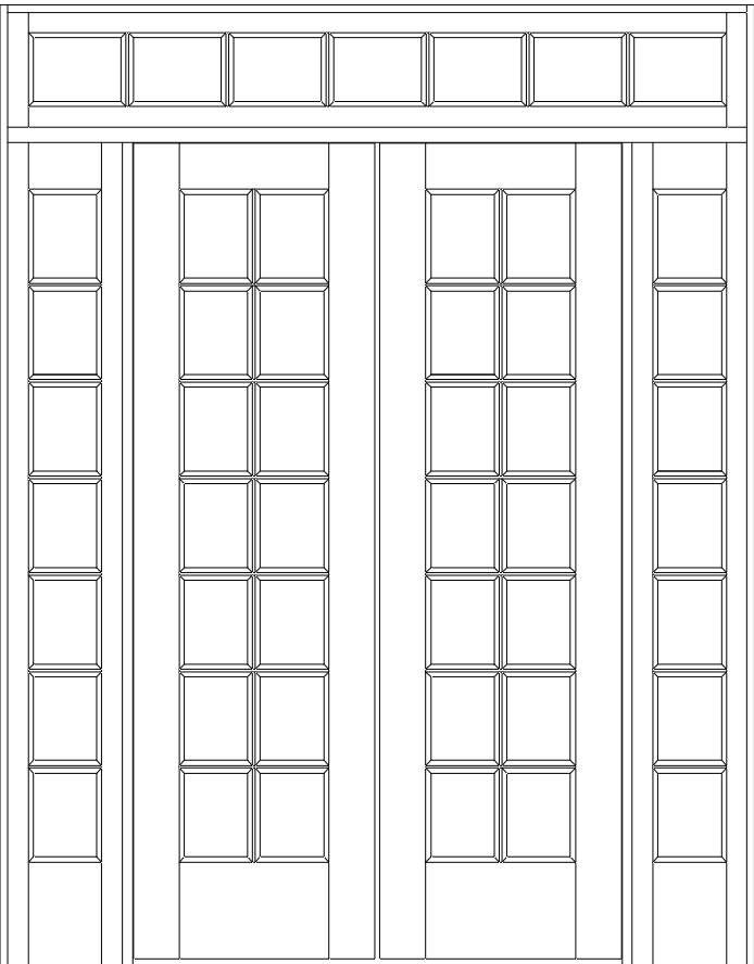
Double Door Unit Doors: 14-Lite T-D-L Sidelights: 7-Lite T-D-L Transom: Rectangle 7-Lite T-D-L
